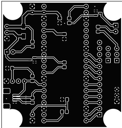
bottom view of top layer
