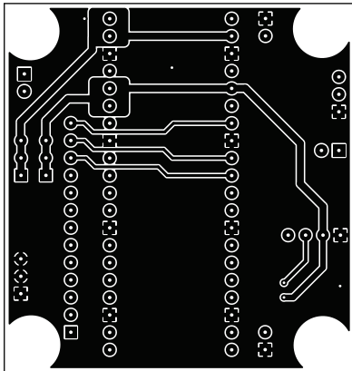
top view of bottom layer
