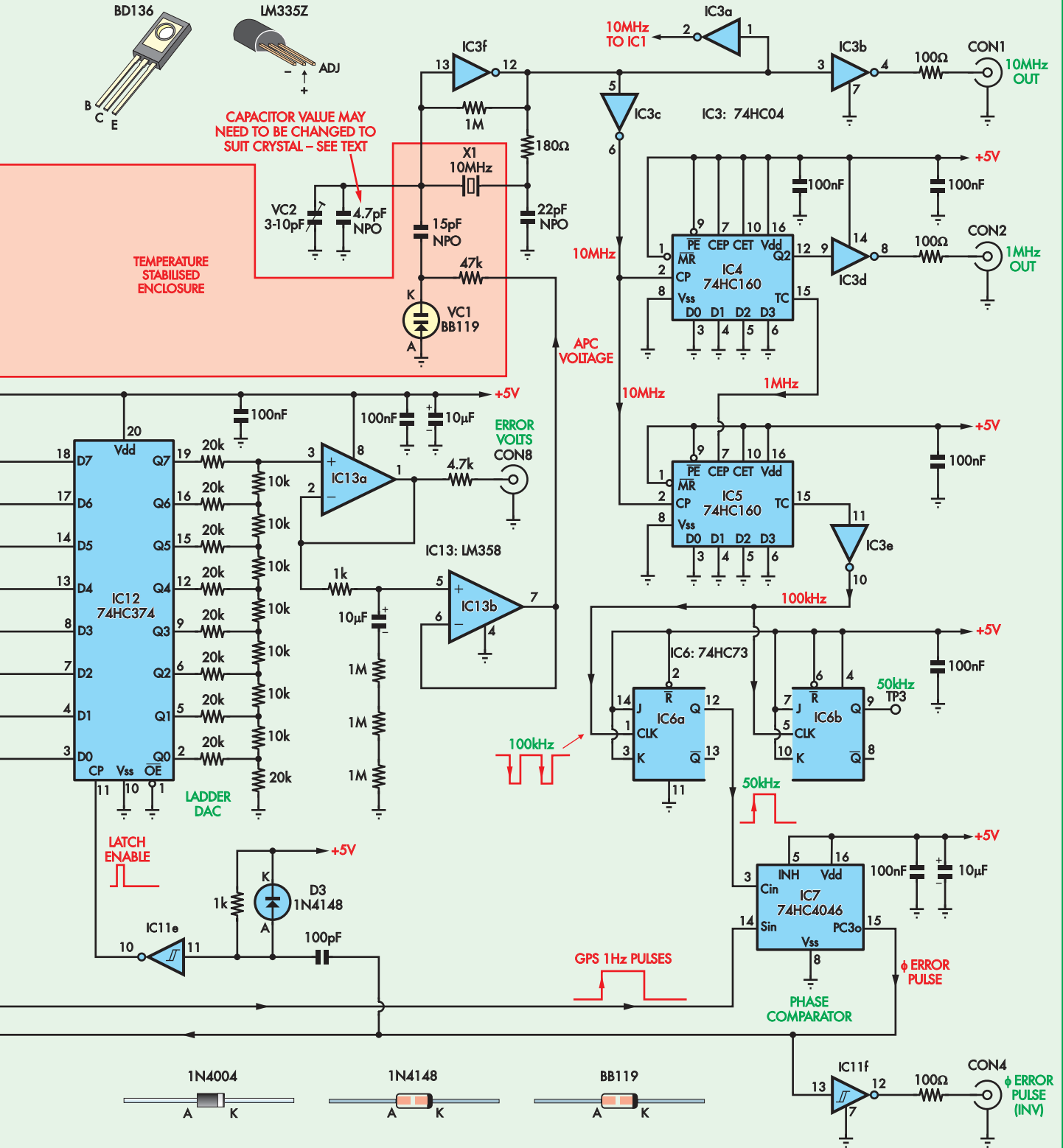
Fig.1(below): the circuit for the modified GPS-Based Frequency Reference. The changes to the original circuit were highlighted on page 41 of the September issue of SILICON CHIP.
